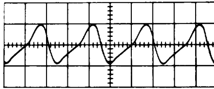
e. Phase Discriminator output, junction of CR1 and R6. Incremental Tuning Oscillator capacitor plates meshed.
