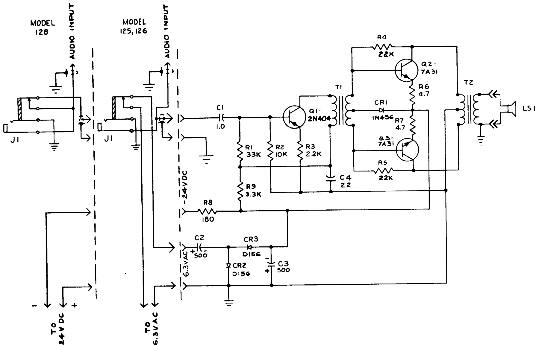
Figure C-7. Universal Speaker Kit Schematic Diagram
