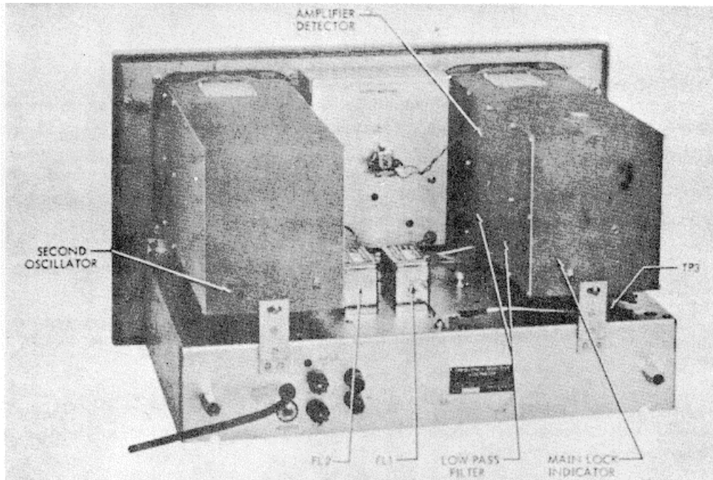
Figure 4-2. Rear View, Module Location
