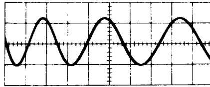
b. Incremental Reference Oscillator and Mixer, Crystal Oscillator output, terminal 2 of transformer T1. Second Oscillator disconnected.
