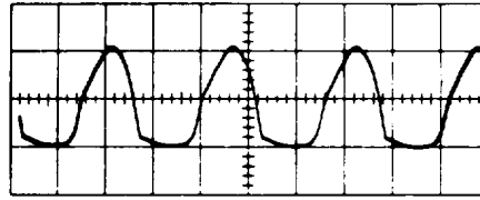
b. Phase Discriminator, terminal 5 of transformer T1. Incremental Tuning Oscillator capacitor plates meshed.
