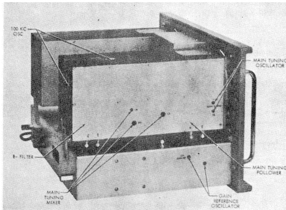
Figure 4-6. Left Side View, Module Location
