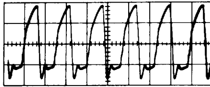
j. First L.F. Amplifier output. Terminal 2 of transformer T1 in Phase Discriminator. Incremental Tuning Oscillator capacitor plates open.
