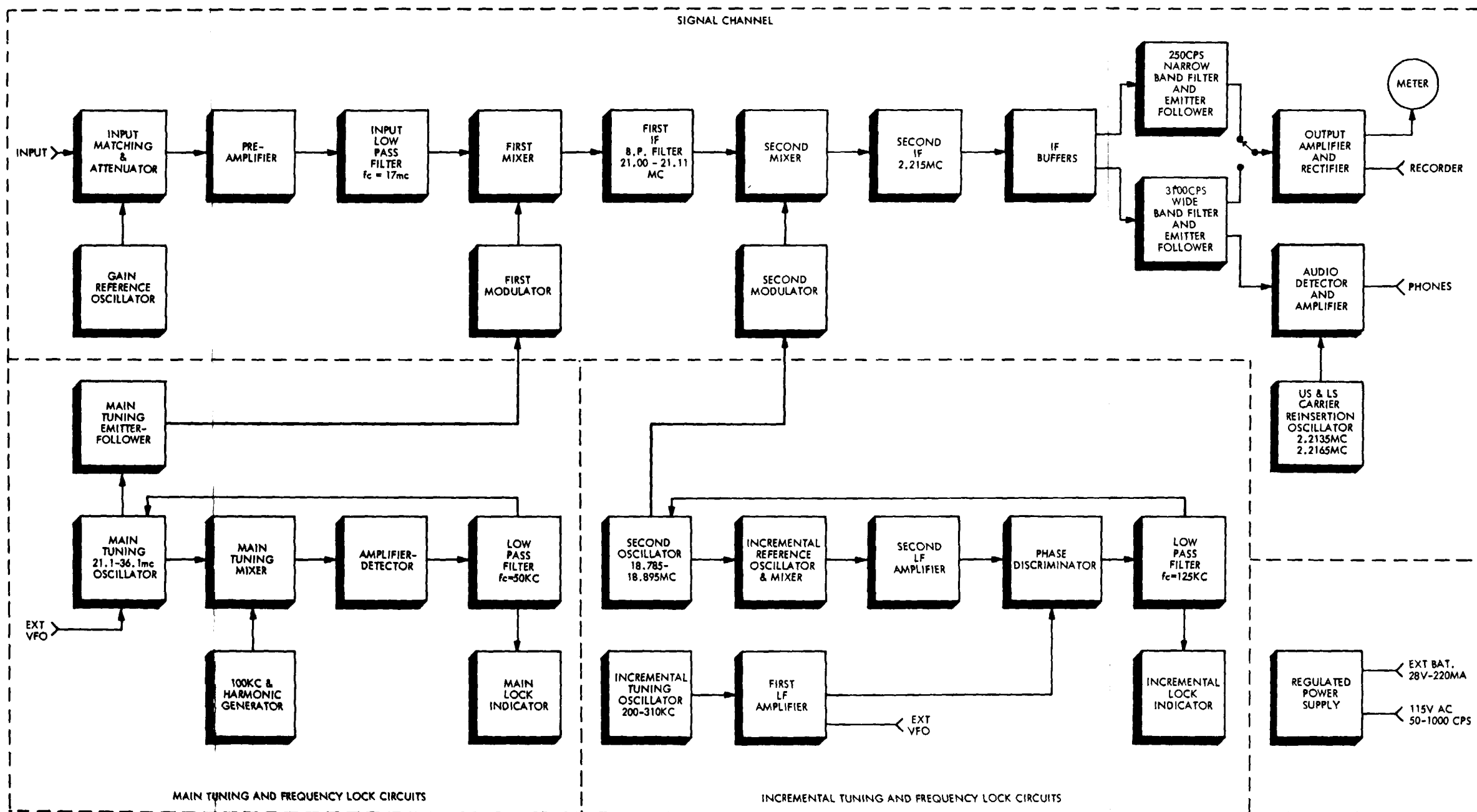
Figure 1-2. Model 128A Block Diagram
