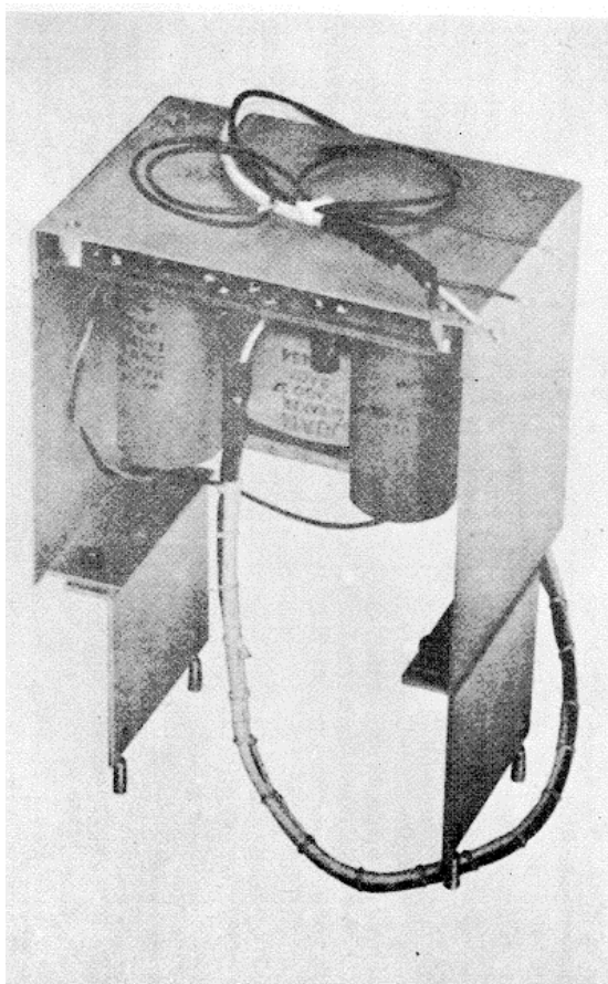
Figure C-1. Speaker Assembly With Model 125/126 Brackets
