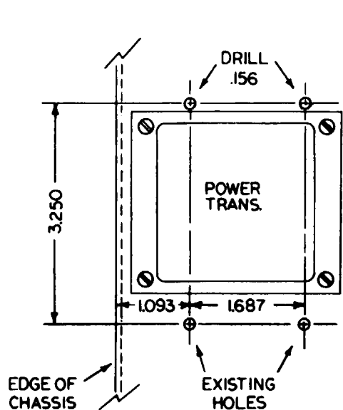
Figure C-3. Mounting Hole Location Model 125/126
