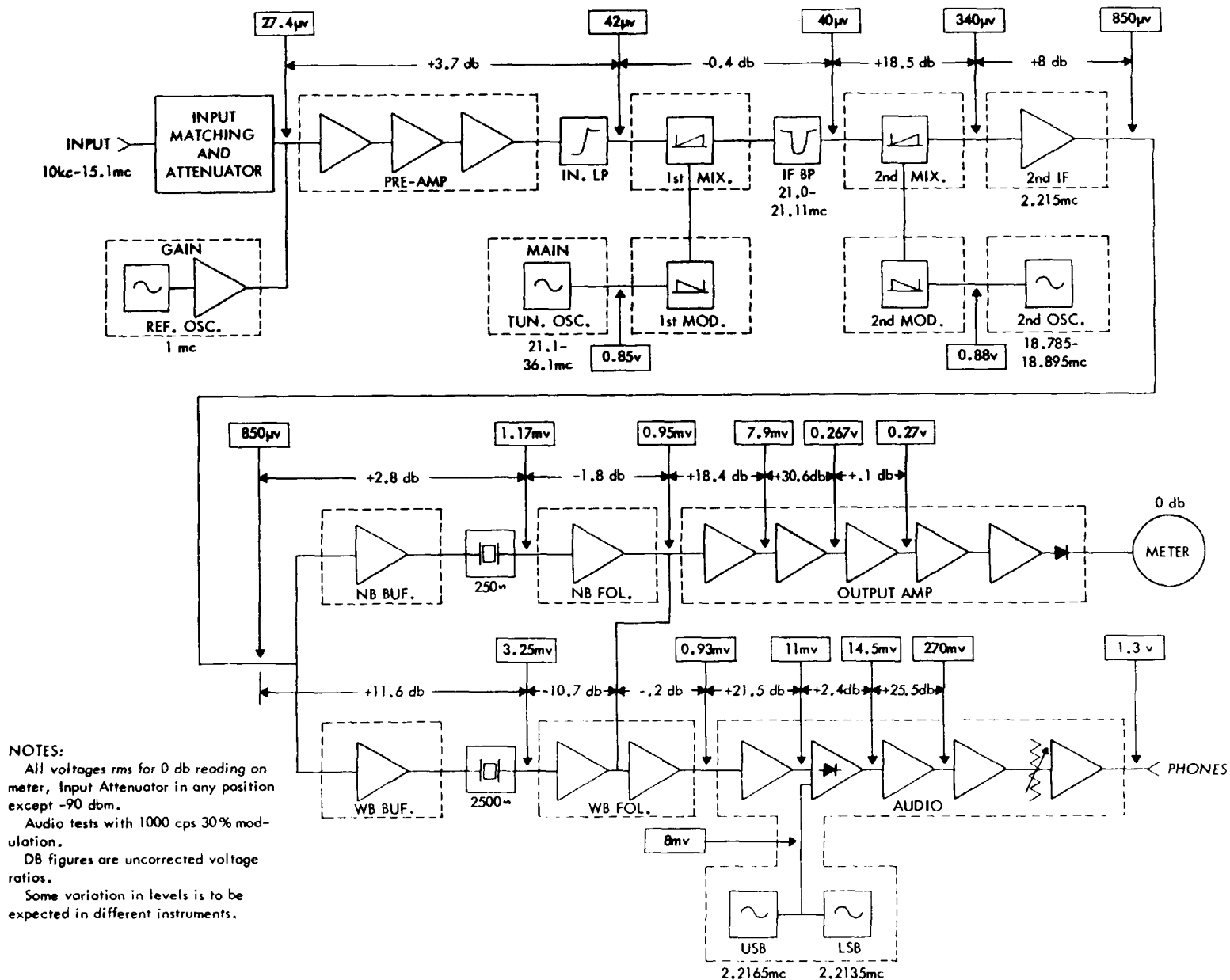
Figure 4-1. Signal Levels, Block Diagram
