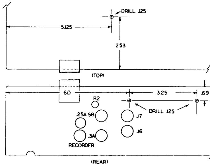
Figure C-4. Mounting Hole Location Model 128
