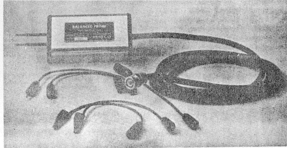
Figure A-1. Balanced Probe With Auxiliary Flexible Leads
