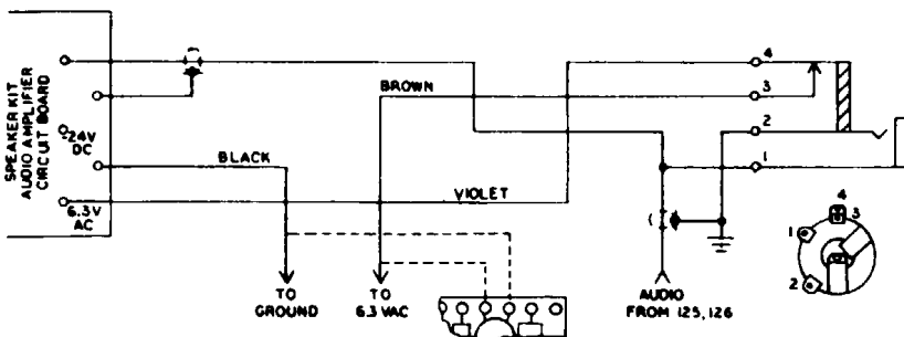
Figure C-5. Wiring Diagram Model 125/126
