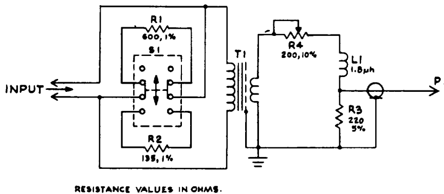
Figure A-2. Model 128-PA Balanced Probe Schematic Diagram
