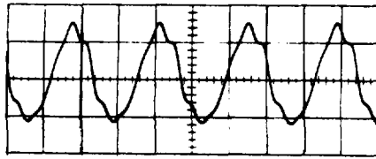
Vert: 1 V/cm Hor: 20 nsec/cm (581 Oscilloscope)
