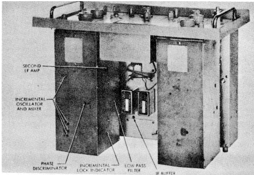
Figure 4-9. Top View, Module Location
